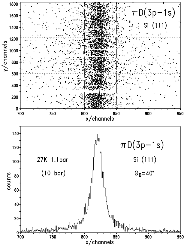
Fig. 7. Top: Scatter plot of the \pi D(3p-1s) reflection measured at a density equivalent to 10 bar (NTP). Its curvature is obtained by a parabola fit. Bottom: projection to the axis of dispersion after curvature correction. One channel (pixel) in the direction of dispersion ( x ) corresponds in first-order reflection to 76.402 \pm 0.001 meV.
