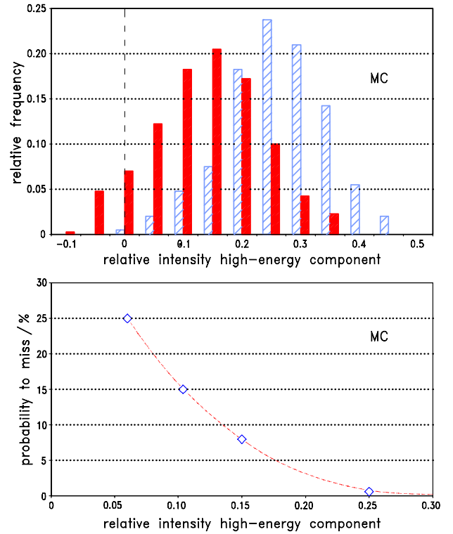
Fig. 10. Top: distributions of relative intensity of a Doppler broadened component induced by the (4-3) Coulomb de-excitation transition found from fits to Monte Carlo (MC) generated spectra. The relative strength used for the simulations is 10% (filled) and 25% (hatched) relative intensity, respectively. In both cases, the result is based on 400 spectra generated for the statistics of the sum of the 10 and 17.5 bar data. Bottom: probability to miss a Doppler contribution corresponding to the (4-3) Coulomb de-excitation (modeled by a uniform kinetic-energy distribution from (76–84) eV) as a function of its relative intensity.
