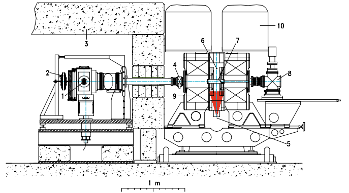
Fig. 4. Sectional drawing of the connection of the cyclotron trap to the crystal chamber of the spectrometer. The symmetry axis of the magnetic field coincides with the line center of the trap to center of the Bragg crystal: 1) Bragg crystal, 2) traction relaxation, 3) concrete shielding, 4) gate valve, 5) X-ray tube (emission cone indicated), 6) position of pion beam without B field, 7) cryogenic target cell including calibration target (right end), 8) target cell support and cryogenic generator, 9) magnet coils of cyclotron trap, 10) LHe dewars.
