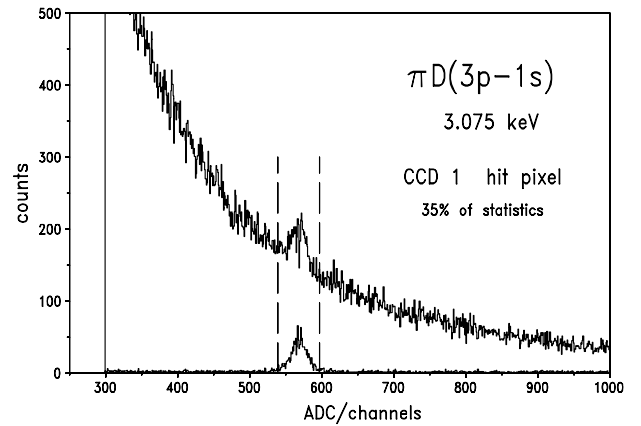
Fig. 6. Spectrum of the collected (digitized) charge in one CCD before and after cluster analysis of one of the 3 CCDs covered by the \pi\text{D}(3p-1s) reflection. Data are from the measurement at 10 bar equivalent density and correspond to 35% of the \pi\text{D} statistics collected with CCD 1. The peak around ADC channel 570 is due to the transition energy of 3.075 keV. Vertical dashed lines indicate the applied “energy cut” of \pm 2.5\sigma allowing for further background reduction.
