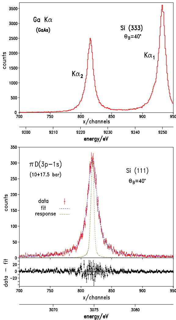
Fig. 8. Top: Ga K\alpha_2 calibration line. The K\alpha_1 component is slightly reduced by the asymmetric emission characteristics of the X-ray tube. Middle: sum spectrum of the \pi D(3p-1s) transition measured at the equivalent densities of 10 and 17.5 bar. The narrow structure represents the response function of the crystal spectrometer (normalised to the height of the measured spectrum). Bottom: residuum of data and fit. The fit is performed without assuming any Doppler components.
