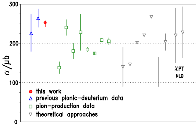
Fig. 14. Threshold parameter \alpha for s -wave pion production compared to results from previous experiments and theoretical studies (from left). Previous X-ray measurements: [47], [45, 46]; pion production and absorption: [144], [145], [146], [147], [148], [150], [151], [152]. Theoretical calculations: [102], [153], [103], [154], [154], [155], [156,157], [67], [68]. Points are given in the same order as listed in table 8.
