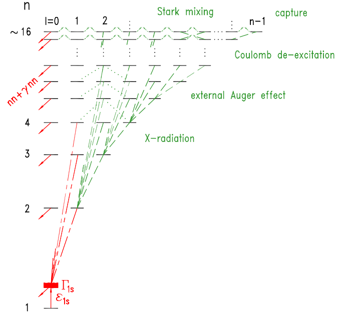
Fig. 1. De-excitation cascade in pionic deuterium. The energy of the X-ray emitted in the \pi\text{D}(3p-1s) transitions is 3.075 keV. Hadronic shift \epsilon_{1s} and width \Gamma_{1s} are of the order of 2.5 and 1 eV, respectively. The hadronic shift is defined as \epsilon_{1s} \equiv E_{\text{exp}} - E_{\text{QED}} , i.e. a negative sign as is the case for \pi\text{D} corresponds to a repulsive interaction.
