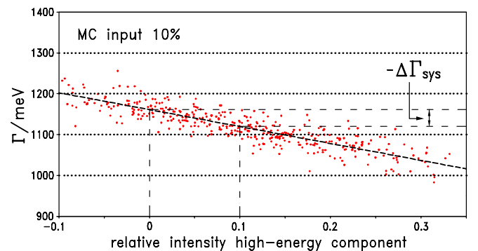
Fig. 11. Distributions of the Lorentz width \Gamma versus the relative intensity of the Doppler broadened component stemming from the (4-3) Coulomb de-excitation. The results are obtained from 400 Monte Carlo simulations performed for the statistics of the sum of the 10 and 17.5 bar data. Input values are 10% relative intensity for the Doppler affected component and 1130 eV for \Gamma .
