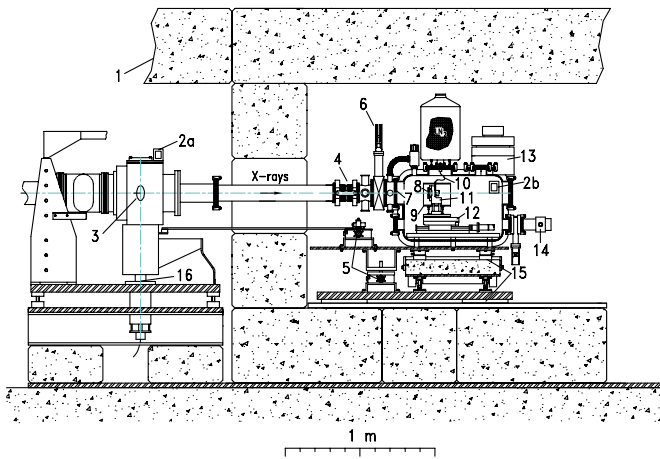
Fig. 5. Sectional drawing of the connection of the crystal chamber to the X-ray detector: 1) concrete shielding, 2a) and 2b) inclination sensors, 3) Bragg crystal, 4) compensator, 5) linear tables for crystal and detector adjustment, 6) gate valve, 7) 5\ \mu\text{m} Mylar window, 8) CCD array, 9) cold trap, 10) copper braid, 11) cold finger, 12) translation table for focal-length adjustment, 13) detector readout electronics, 14) turbomolecular pump, 15) air cushion support, 16) crystal chamber support.
