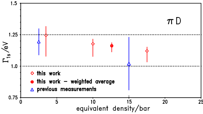
Fig. 13. Experimental information on the hadronic broadening in pionic deuterium. Previous measurements were performed at 2.5 bar [47] and 15 bar [45,46] equivalent density.
