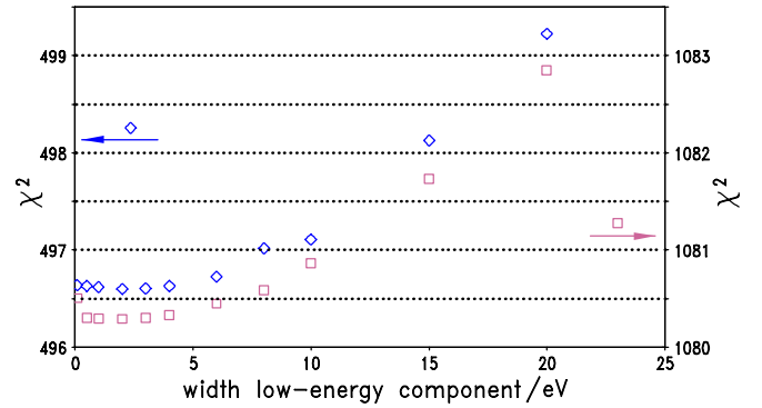
Fig. 9. Search for evidence of an extended low-energy component in the kinetic-energy distribution by including in the fit of the data a uniform kinetic-energy distribution of variable width starting at T_{\text{kin}} = 0 . Allowing for kinetic energies above about 8 eV increasingly downgrades the quality of the fit. Diamonds (left \chi^2 scale) are due to the 10 bar data. Squares (right scale) are from a combined fit to the two spectra taken at 10 and 17.5 bar. Degrees of freedom in the fits are 487 (left scale) and 974 (right).
