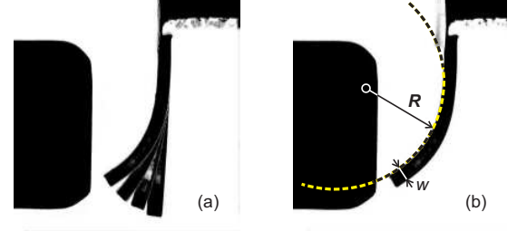
Fig. 3. (a) A composite image showing the extent of cantilever bending. On the left one can see the tip of the soldering iron. (b) The scheme of the manual analysis of the cantilever curvature.
