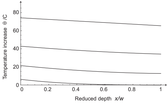
Fig. 4. Plots of \theta = T - T_0 across the cantilever thickness x/w . Increasing curves are for the times Dt/w^2 = 0.1, 1, 3 and 100 .
