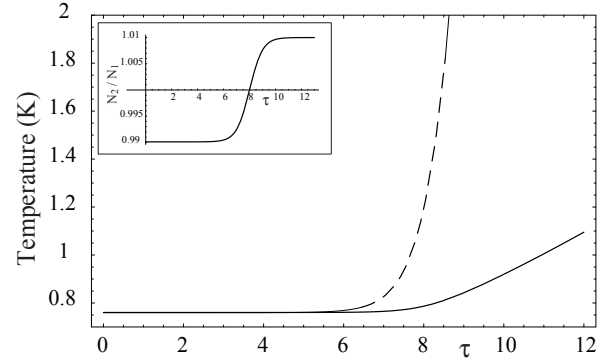
Fig. 5. Time evolution of the temperature of the system for A' = 1 (dotted line) and A' = 0.05 (solid line). For both graphics we have set \omega_0 = 10^{14} Hz and n_B = B/A = 10^3 . The box in the top left corner is the ratio between the populations of the two-level atoms. This quantity does not depend on A' and B' separately, but on the ratio n_B = B/A only [see Eqs. (13) and (14)].
